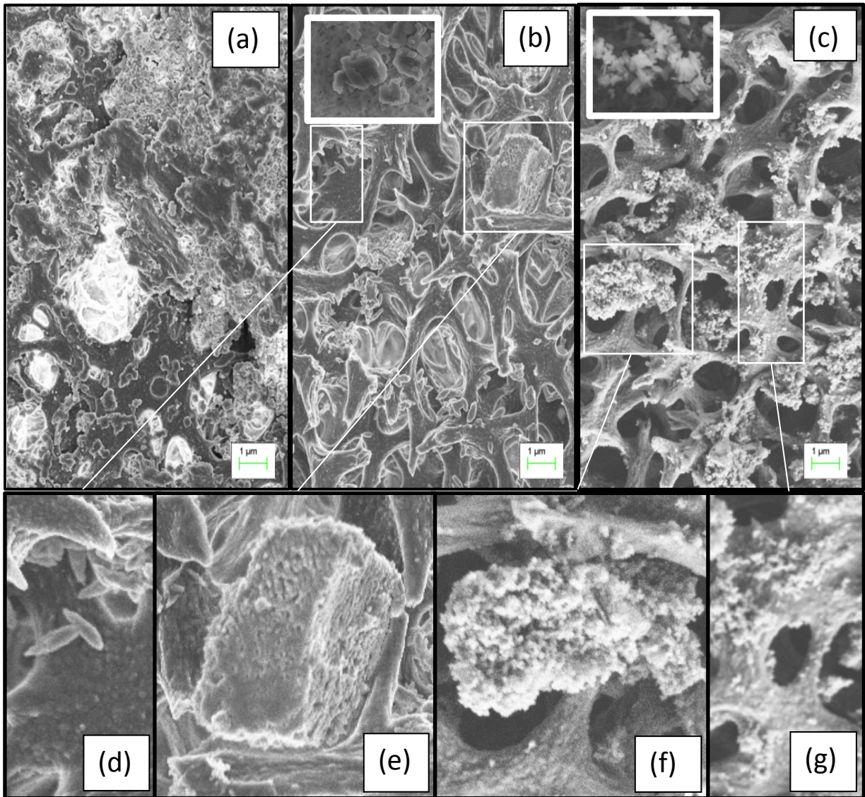
Figure 5: SEM image of the solid produced at high Mg (15.2 mM) and high \text{CO}_3 (30.6 mM), in the presence of phosphate (56 mg/L) on a cellulose acetate 0.45 micron filter used to remove the solids from the mother liquor : (a) in the absence of added seed; (b) in the presence of \text{CaCO}_3 seed; (c) in the presence of \text{CaHPO}_4 seed; (d) detail from image 5(b) showing calcium aragonite-like crystals, (e) detail from image 5(b) showing cubic calcium carbonate seed crystal with thin layer of precipitate; (f) detail from image 5(c) showing what appears to be precipitated material on \text{CaHPO}_4 seed; (g) detail of image 5(c) showing traces of fine precipitate on the membrane material. The inserts in images 5(b) and 5(c) are low magnification images of \text{CaCO}_3 seed and \text{CaHPO}_4 seed respectively.
