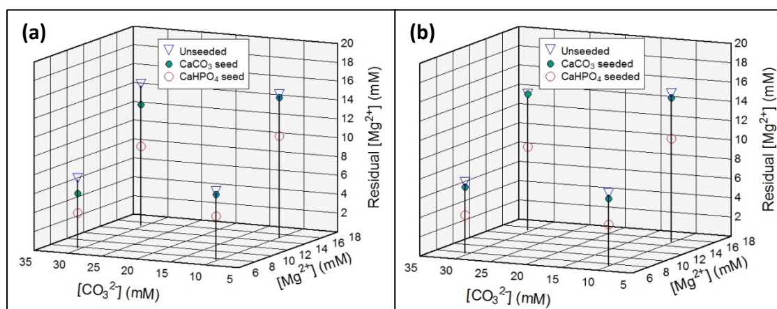
Figure 3: Residual magnesium concentrations in the absence (a) and in the presence (b) of phosphate at various starting magnesium and carbonate levels
